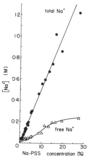
FIGURE 7. The concentration of total Na^+ and free Na^+ in increasing concentration of Na^+ poly-styrene sulfonate (NaPSSP.) The abscissa represents concentration of NaPSS as percentage of solution (weight in g. /volume in ml.) Free Na^+ was detected by a Na^+ -selective glass electrode. (from Ling and Zhang 1983)
